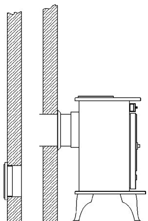
Rear flue connection into the chimney with sealing collar. Cleaning door on opposite side.
