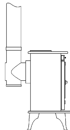
Rear outlet connected to top outlet by 'T' piece with cleaning door, to bring stove forward.
